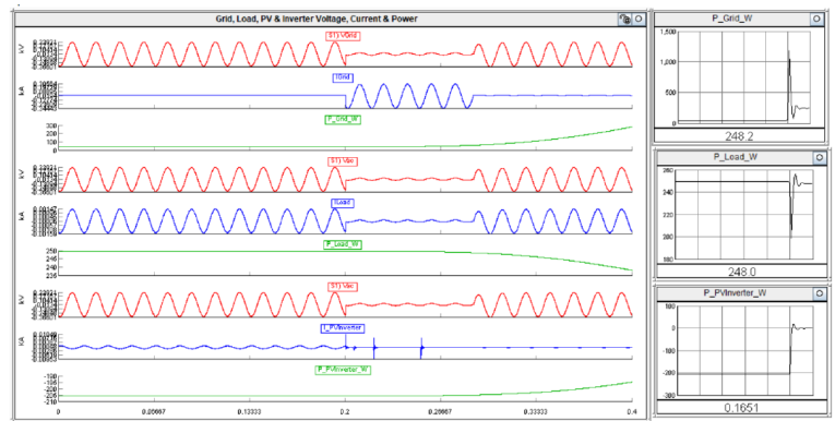
Simulation results for power-hardware-in-the-loop testing of a PV microinverter for a 5 cycle L-G fault
