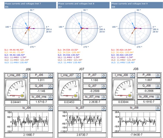
Steady-state feeder current and voltage values measured by the SSC600 (top) are compared to theoretical values from the real-time simulation (bottom)
